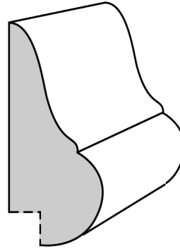
▲ F706R - 11/16" X 1 5/8" w/ 1/4" x 1/4" Rabbet
